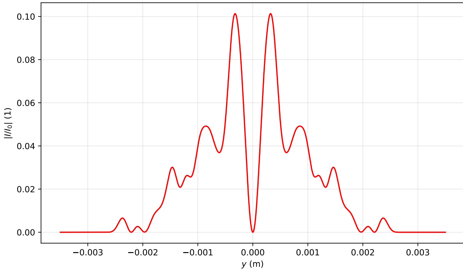
Intensity profile I(x=0, y, z=2.388)/I_0 , P_{in}=8.0P_{cr} , artificial time
